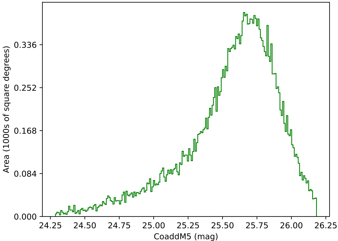
too_elab_r64_d2_giz_v3.4_10yrs Yr 1 g band: CoaddM5
