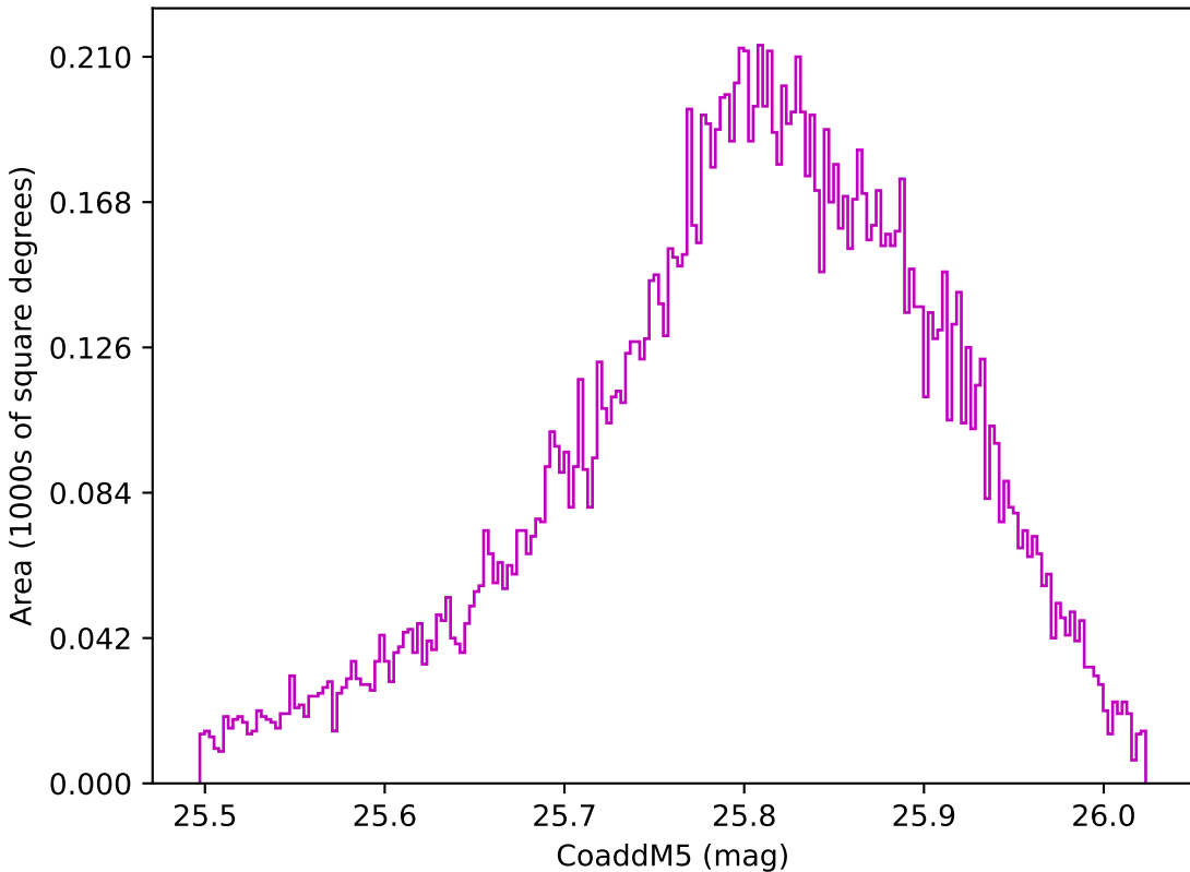
too_elab_r64_d2_giz_v3.4_10yrs WFD z band: CoaddM5
