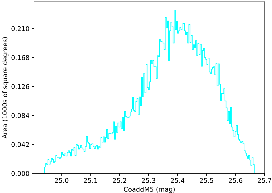
too_elab_r64_d2_giz_v3.4_10yrs WFD u band: CoaddM5
