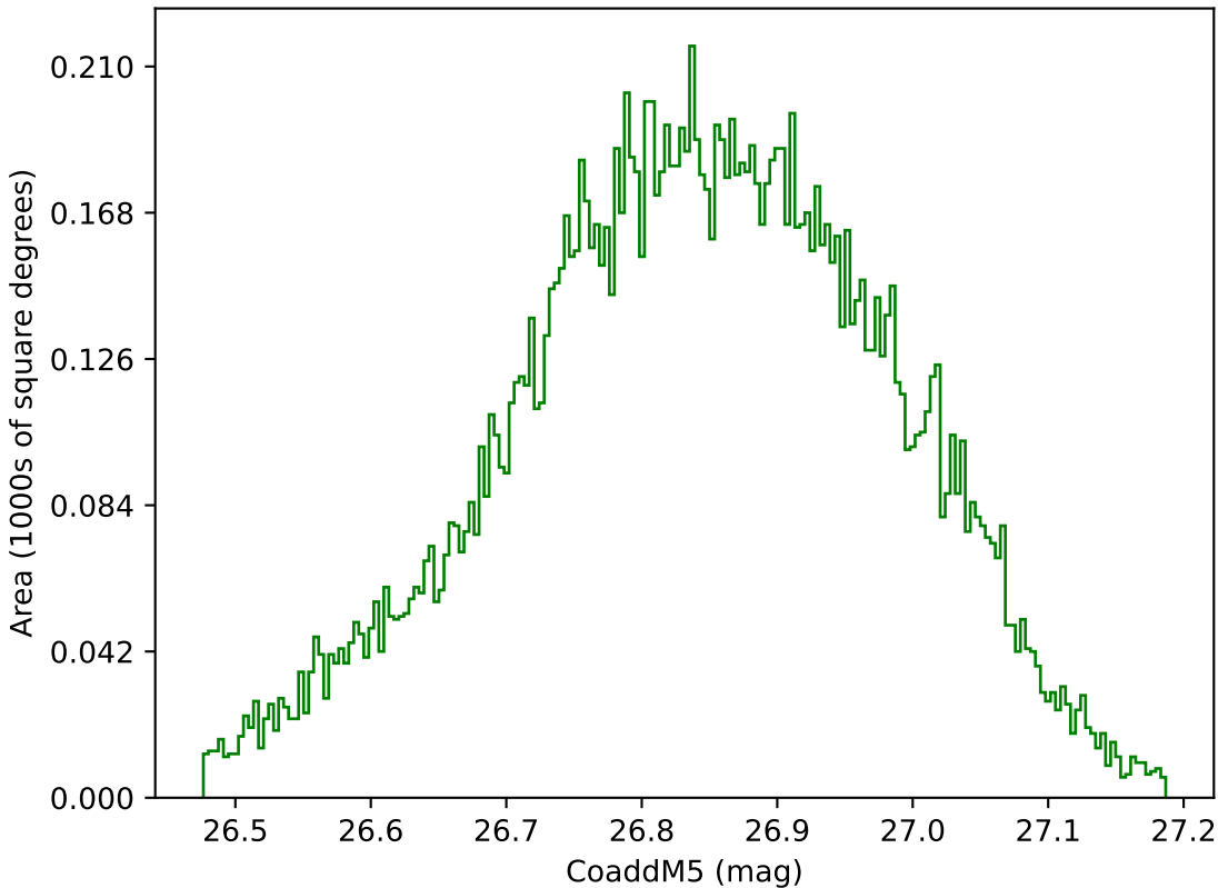
too_elab_r64_d2_giz_v3.4_10yrs WFD g band: CoaddM5
