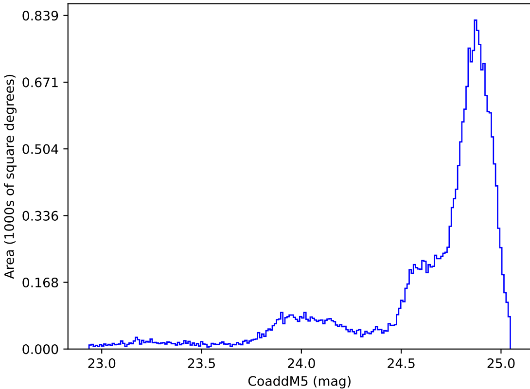
too_elab_r64_d2_giz_v3.4_10yrs All sky y band: CoaddM5
