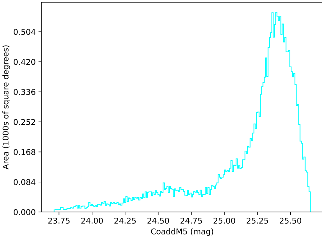
too_elab_r64_d2_giz_v3.4_10yrs All sky u band: CoaddM5
