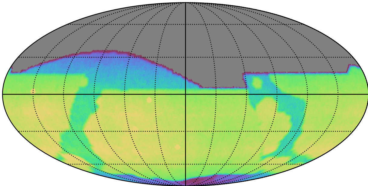
too_elab_r64_d2_giz_v3.4_10yrs All sky r band: CoaddM5
