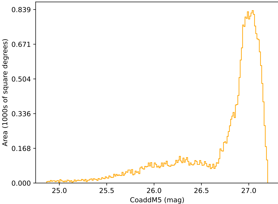
too_elab_r64_d2_giz_v3.4_10yrs All sky r band: CoaddM5
