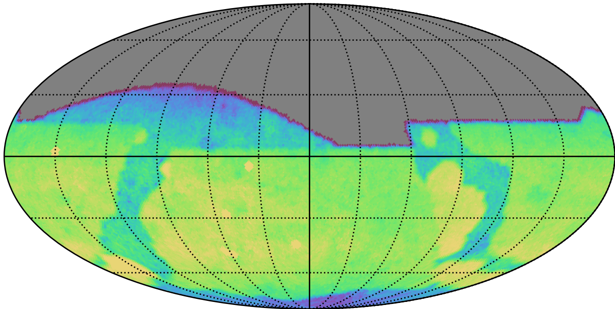
too_elab_r64_d2_giz_v3.4_10yrs All sky g band: CoaddM5
