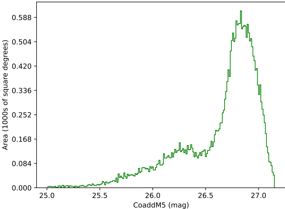
too_elab_r64_d2_giz_v3.4_10yrs All sky g band: CoaddM5
