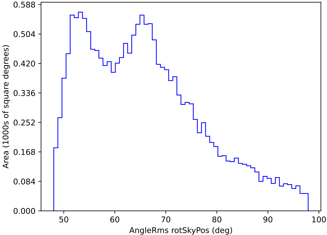
too_elab_r64_d2_giz_v3.4_10yrs WFD r band: AngleRms rotSkyPos
