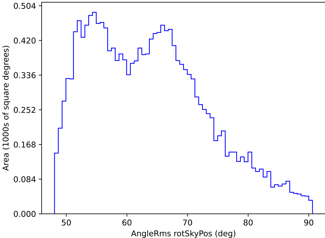
too_elab_r64_d2_giz_v3.4_10yrs WFD i band: AngleRms rotSkyPos
