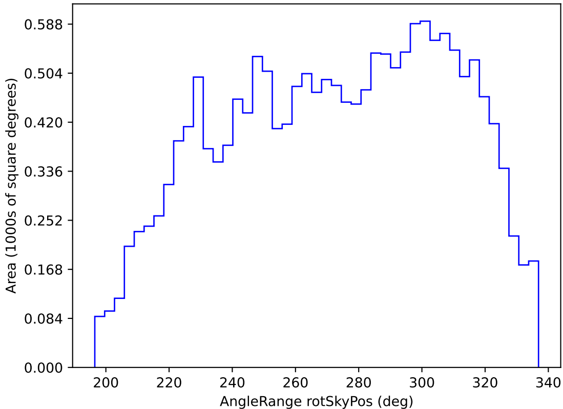
too_elab_r64_d2_giz_v3.4_10yrs WFD y band: AngleRange rotSkyPos
