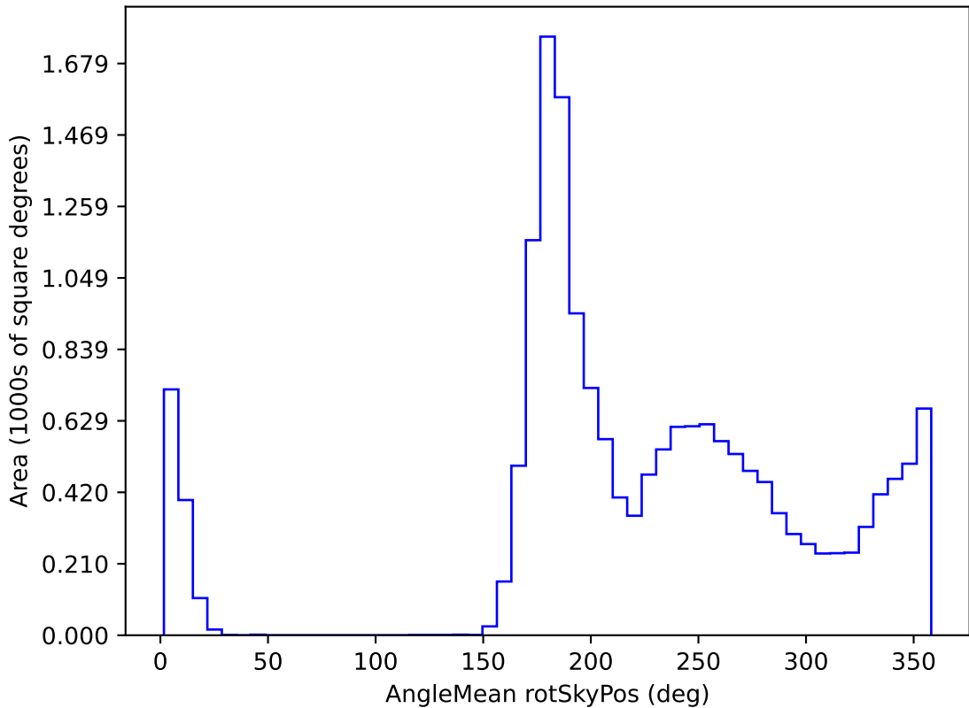
too_elab_r64_d2_giz_v3.4_10yrs WFD y band: AngleMean rotSkyPos
