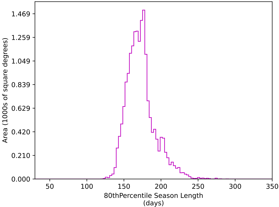
too_elab_r64_d2_giz_v3.4_10yrs WFD z band: 80thPercentile Season Length
