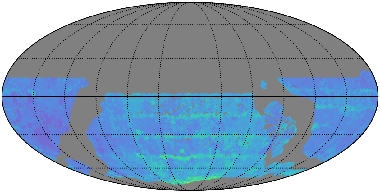
too_elab_r64_d2_giz_v3.4_10yrs WFD y band: 80thPercentile Season Length
