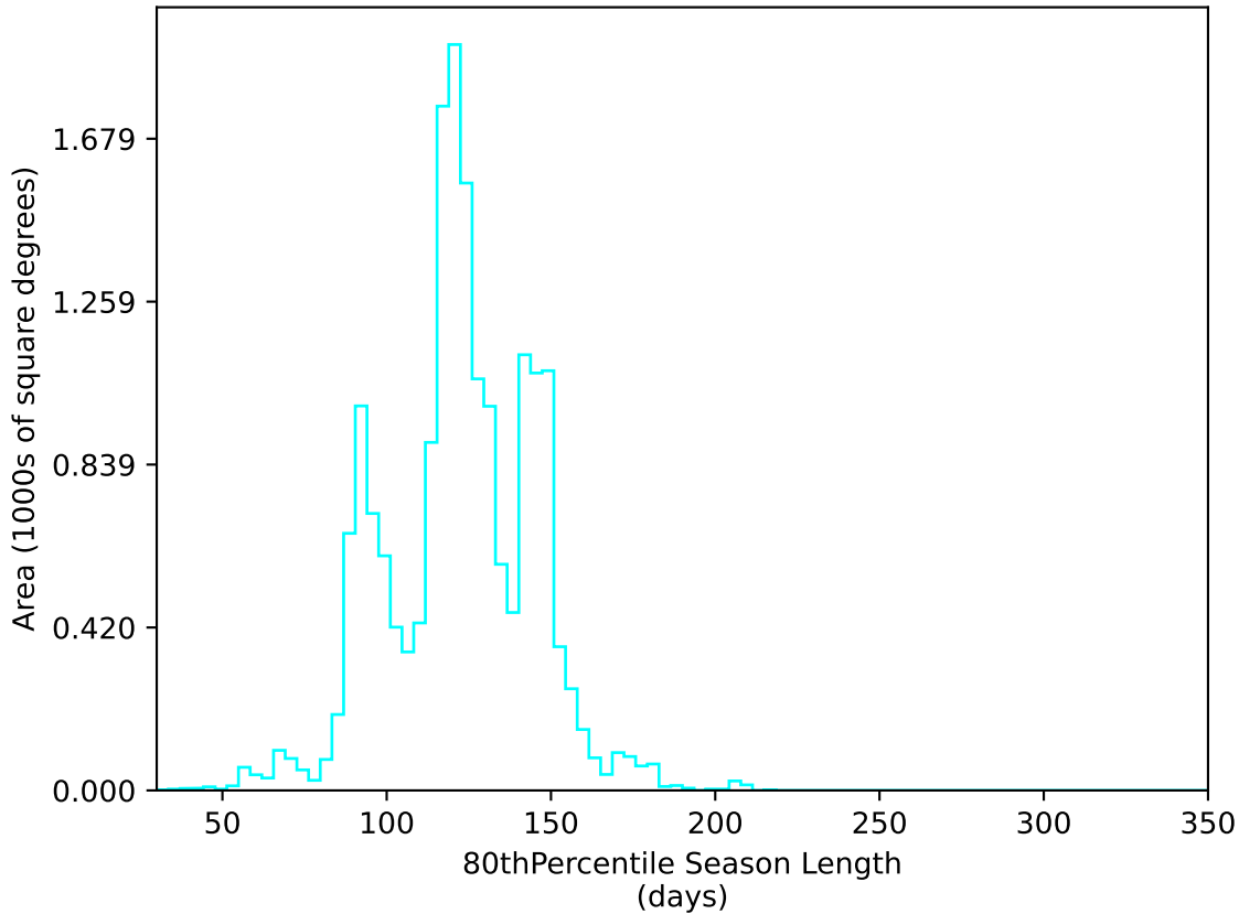
too_elab_r64_d2_giz_v3.4_10yrs WFD u band: 80thPercentile Season Length
