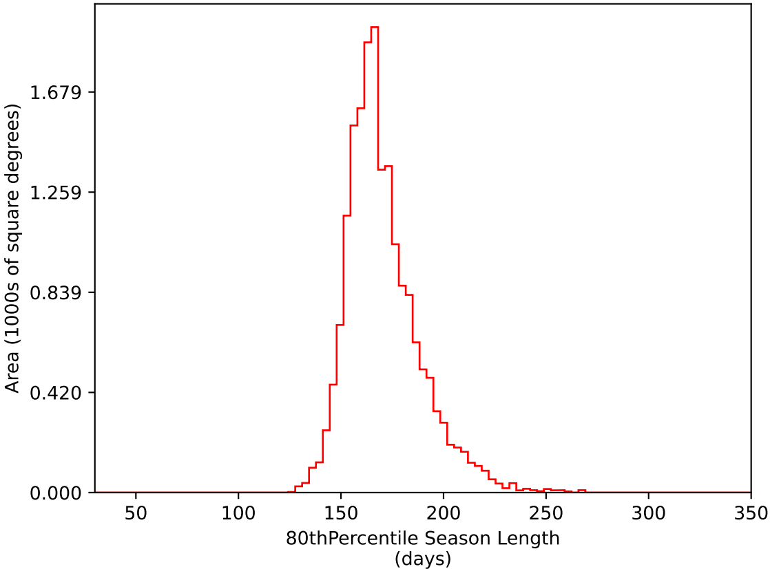
too_elab_r64_d2_giz_v3.4_10yrs WFD i band: 80thPercentile Season Length
