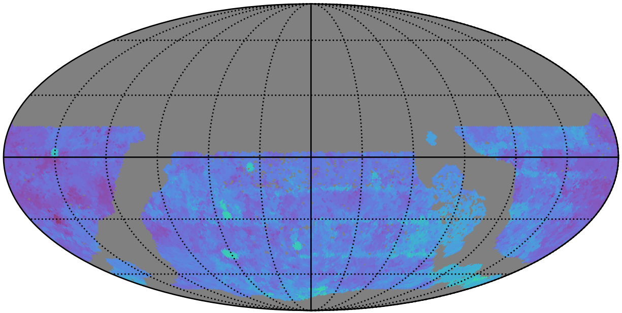
too_elab_r64_d2_giz_v3.4_10yrs WFD g band: 80thPercentile Season Length
