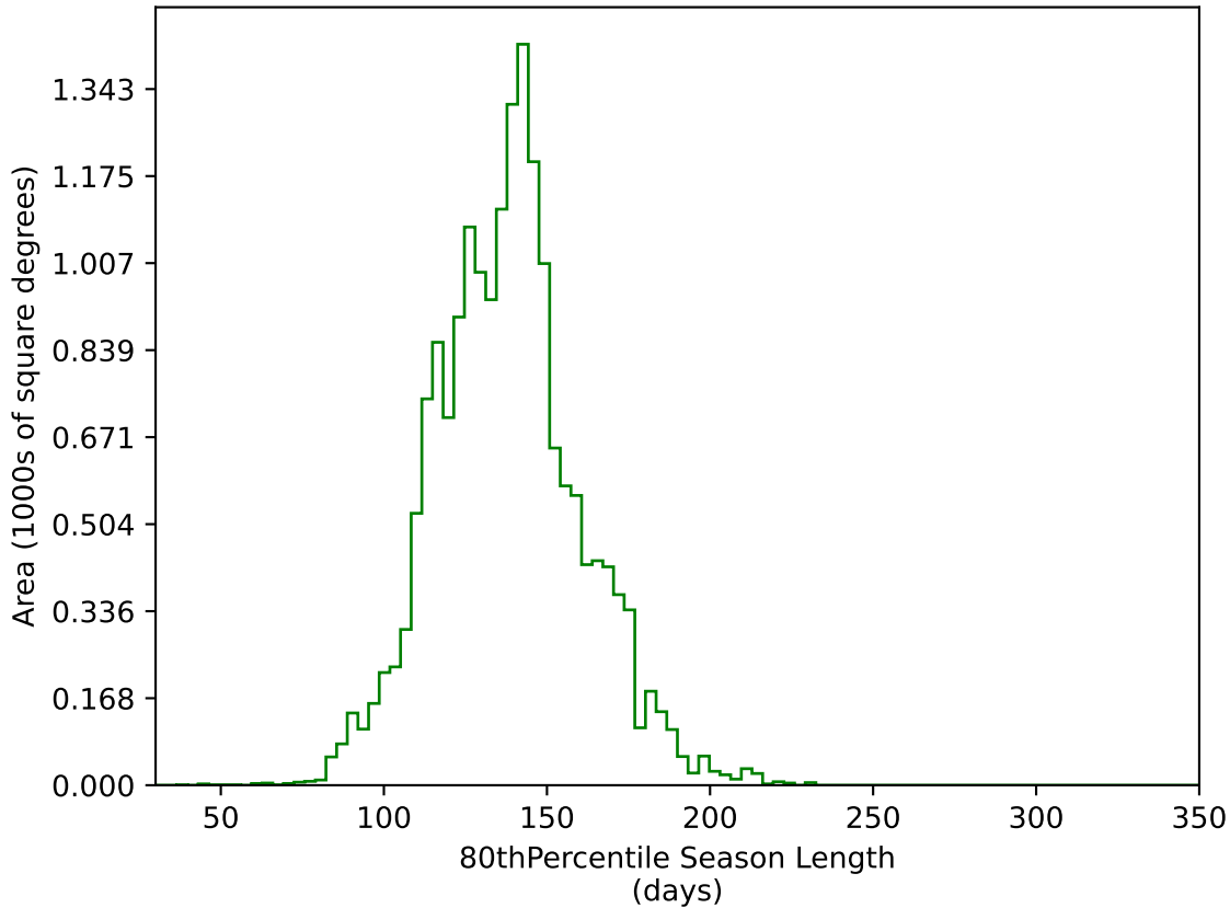
too_elab_r64_d2_giz_v3.4_10yrs WFD g band: 80thPercentile Season Length
