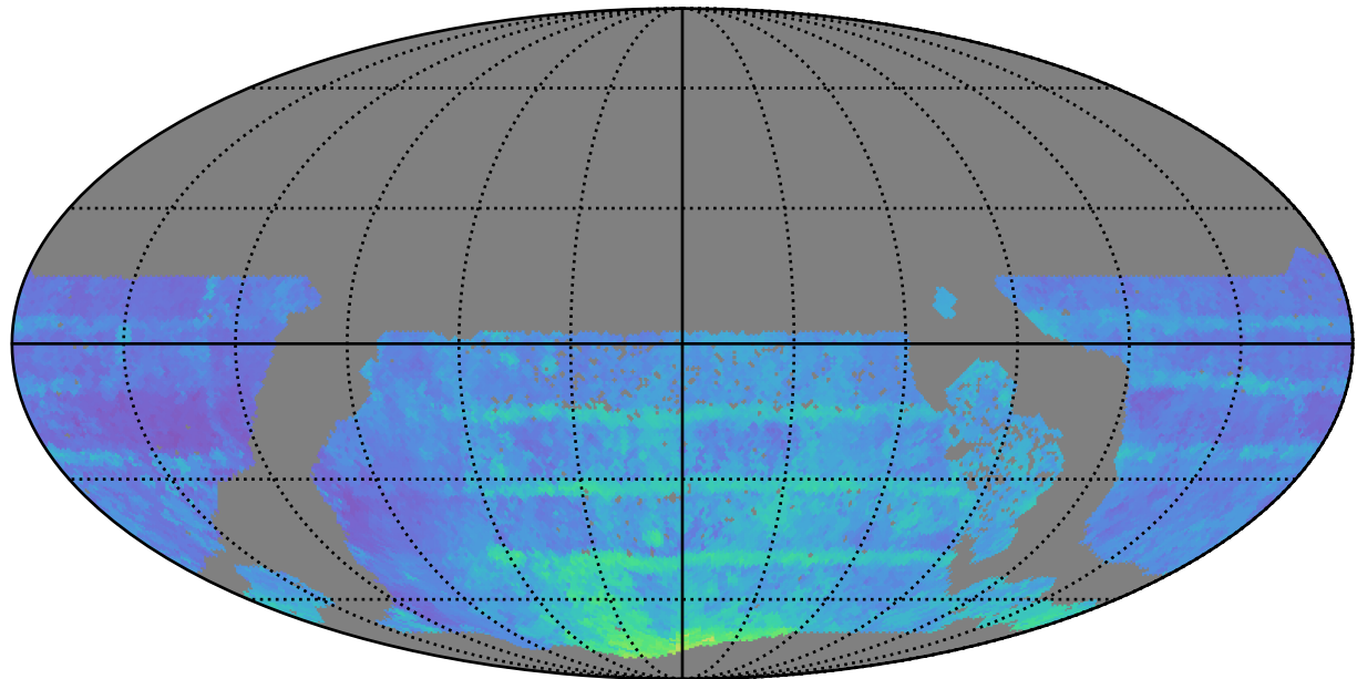
too_elab_r64_d2_giz_v3.4_10yrs WFD all bands: 80thPercentile Season Length
