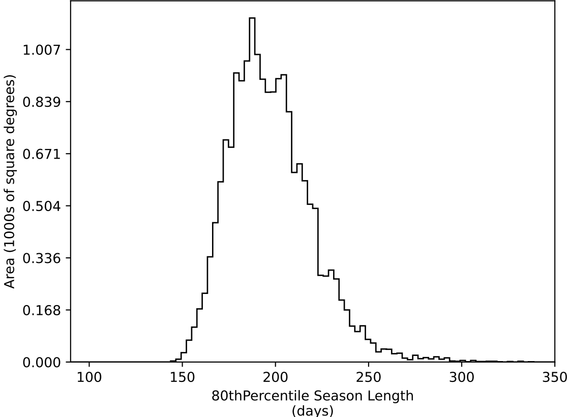
too_elab_r64_d2_giz_v3.4_10yrs WFD all bands: 80thPercentile Season Length
