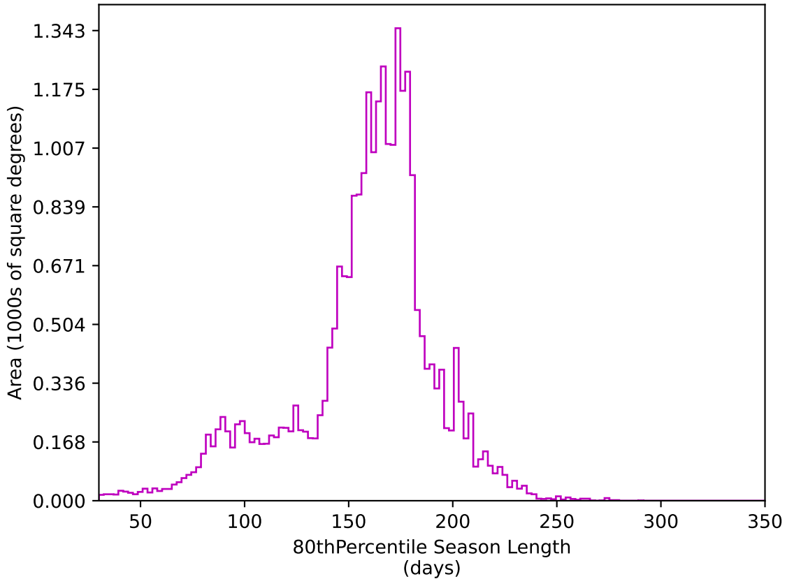
too_elab_r64_d2_giz_v3.4_10yrs All sky z band: 80thPercentile Season Length
