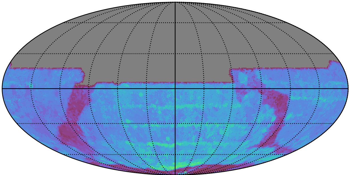
too_elab_r64_d2_giz_v3.4_10yrs All sky y band: 80thPercentile Season Length
