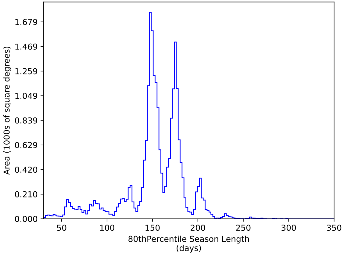
too_elab_r64_d2_giz_v3.4_10yrs All sky y band: 80thPercentile Season Length
