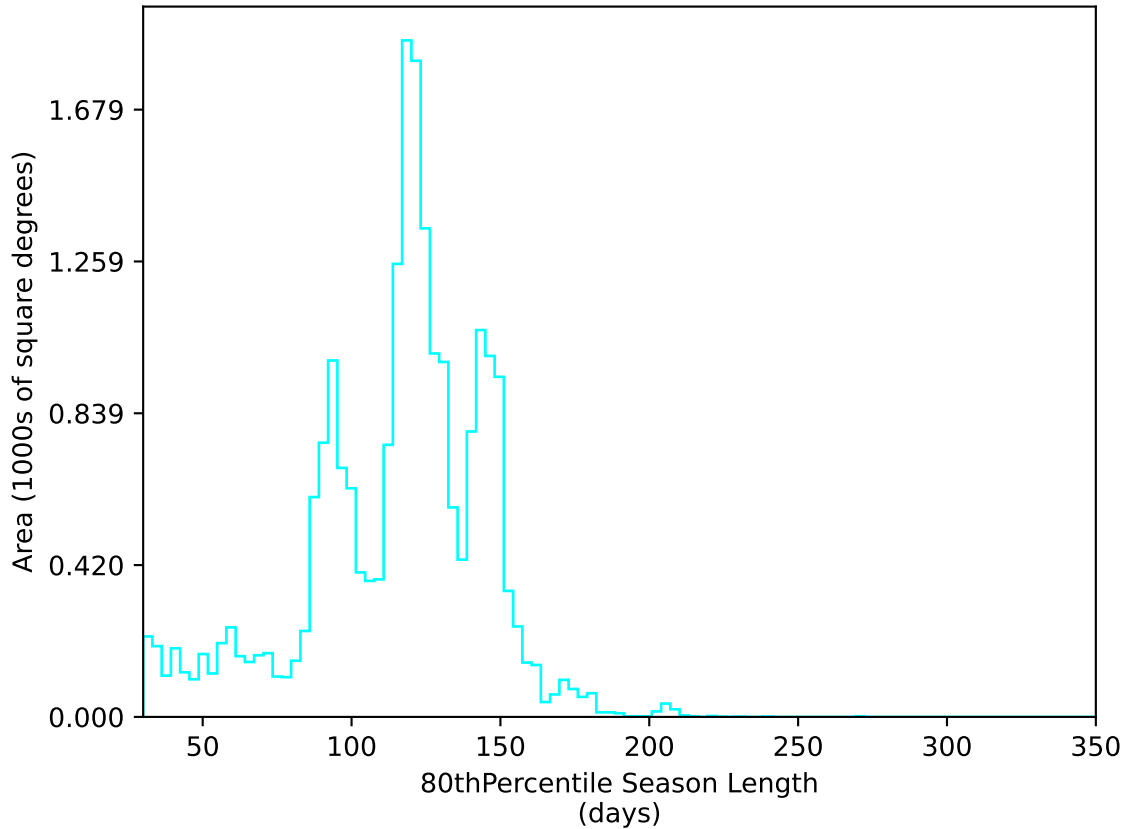
too_elab_r64_d2_giz_v3.4_10yrs All sky u band: 80thPercentile Season Length
