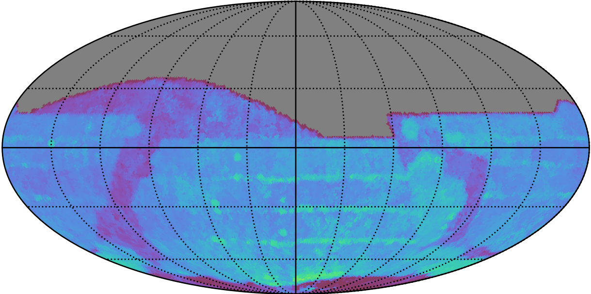
too_elab_r64_d2_giz_v3.4_10yrs All sky r band: 80thPercentile Season Length
