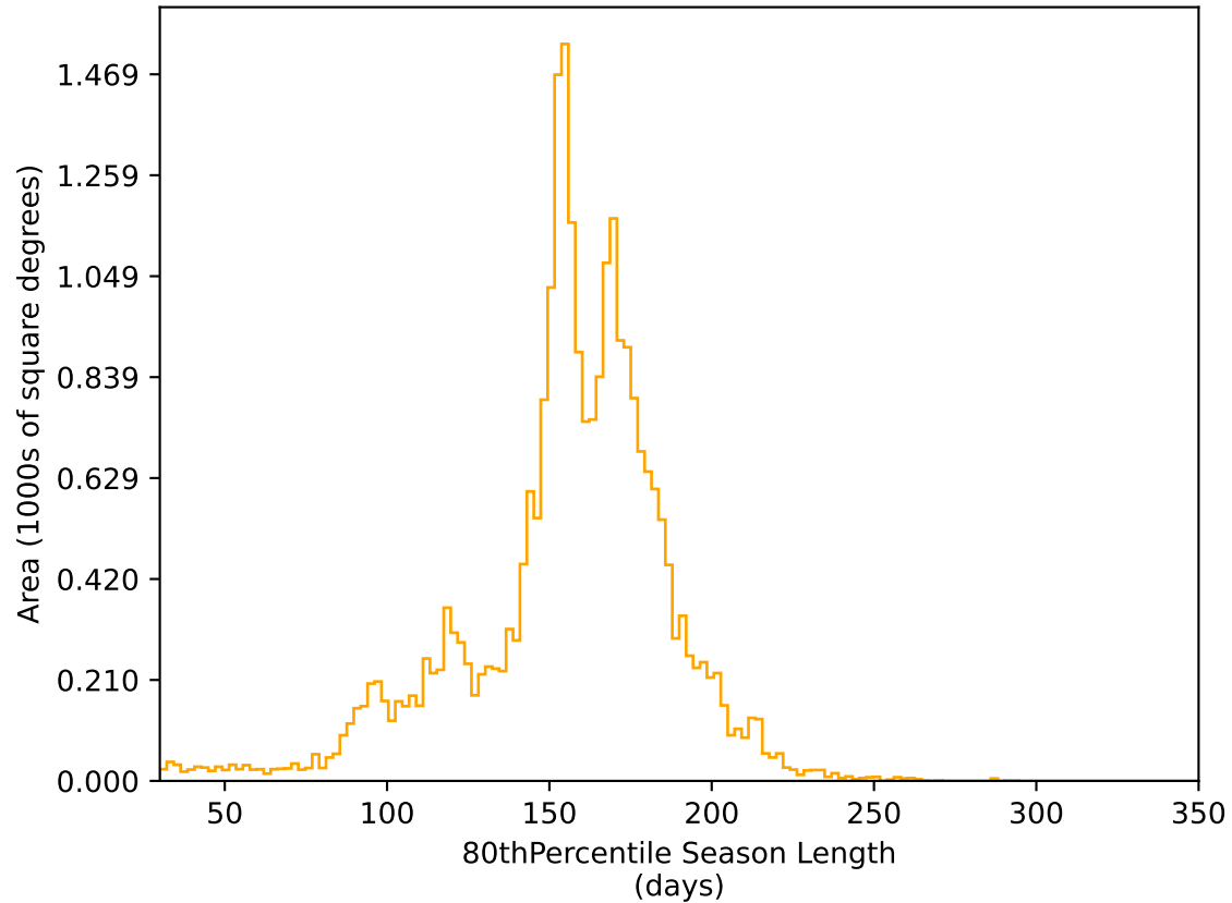
too_elab_r64_d2_giz_v3.4_10yrs All sky r band: 80thPercentile Season Length
