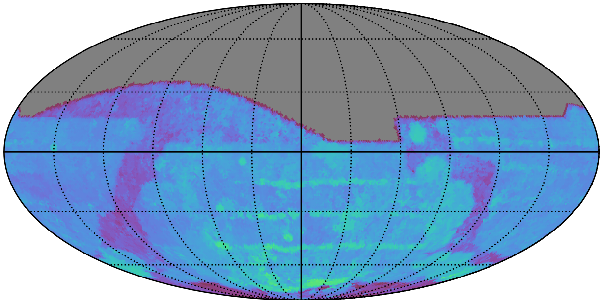
too_elab_r64_d2_giz_v3.4_10yrs All sky i band: 80thPercentile Season Length
