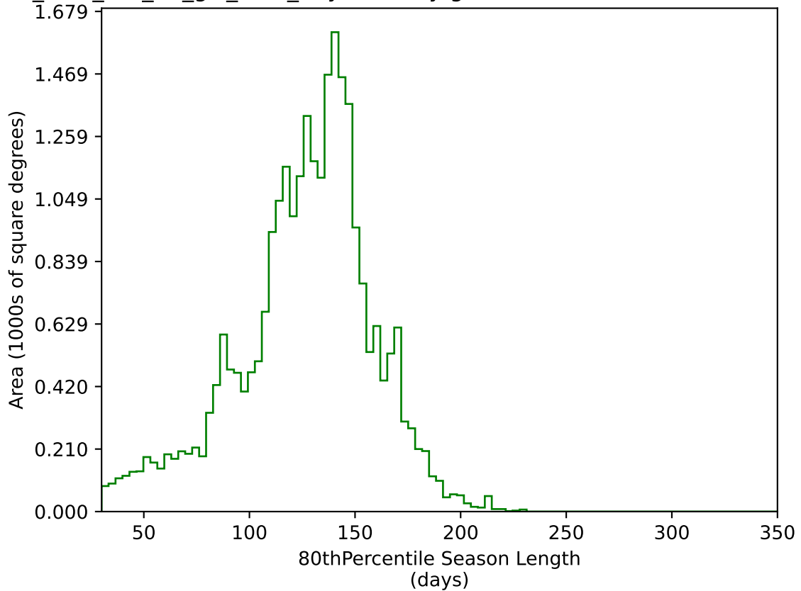
too_elab_r64_d2_giz_v3.4_10yrs All sky g band: 80thPercentile Season Length
