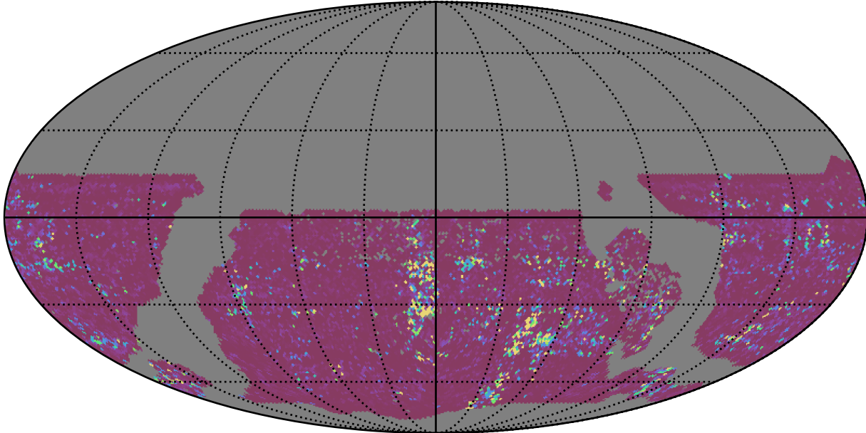
too_elab_r64_d2_giz_v3.4_10yrs WFD u band: 75th Percentile Intranight Timespan
