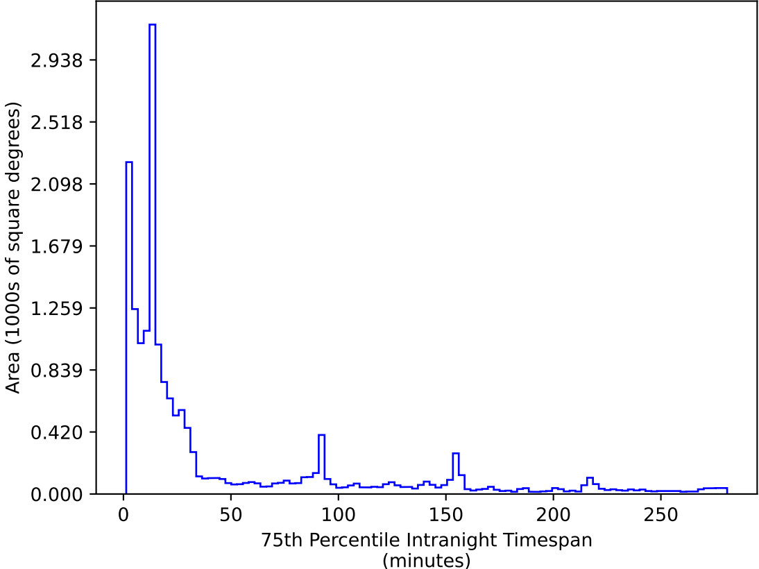
too_elab_r64_d2_giz_v3.4_10yrs WFD r band: 75th Percentile Intranight Timespan
