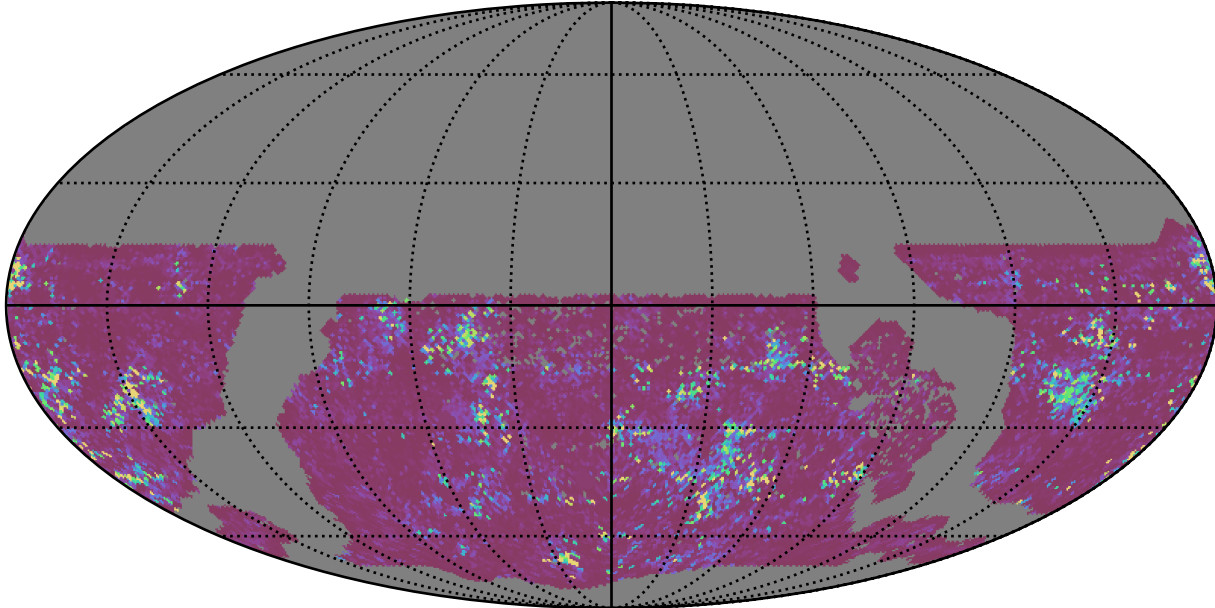
too_elab_r64_d2_giz_v3.4_10yrs WFD g band: 75th Percentile Intranight Timespan
