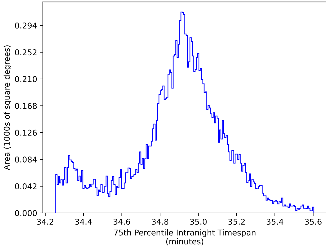
too_elab_r64_d2_giz_v3.4_10yrs WFD: 75th Percentile Intranight Timespan
