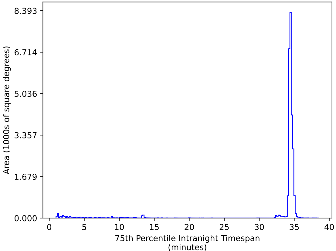
too_elab_r64_d2_giz_v3.4_10yrs All sky zy bands: 75th Percentile Intranight Timespan
