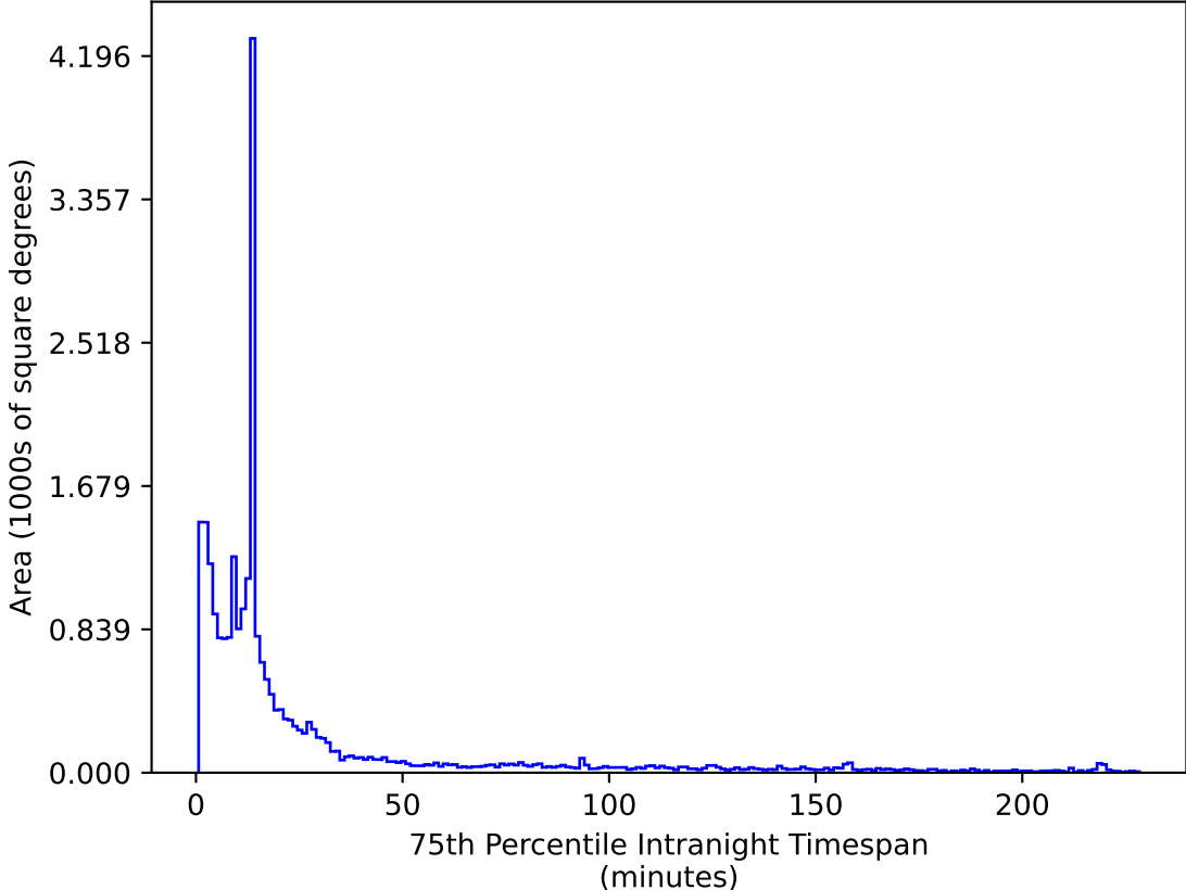
too_elab_r64_d2_giz_v3.4_10yrs All sky z band: 75th Percentile Intranight Timespan
