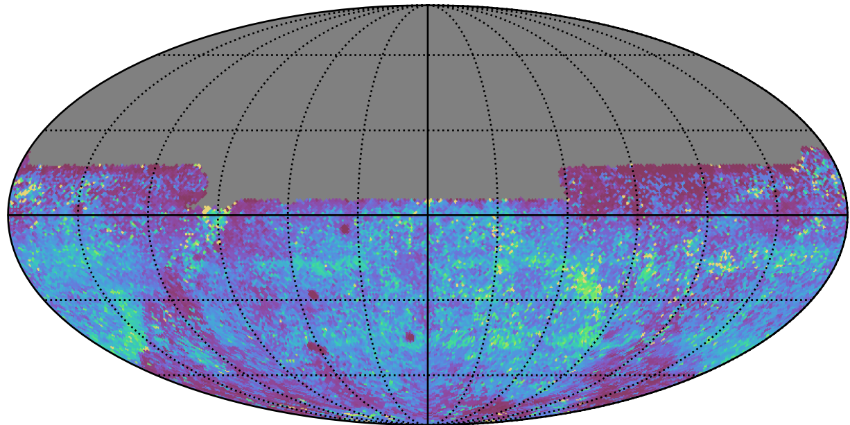
too_elab_r64_d2_giz_v3.4_10yrs All sky y band: 75th Percentile Intranight Timespan
