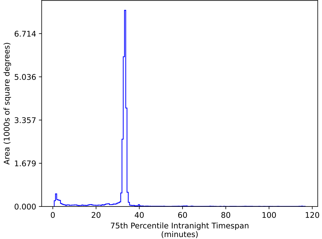
too_elab_r64_d2_giz_v3.4_10yrs All sky ug bands: 75th Percentile Intranight Timespan
