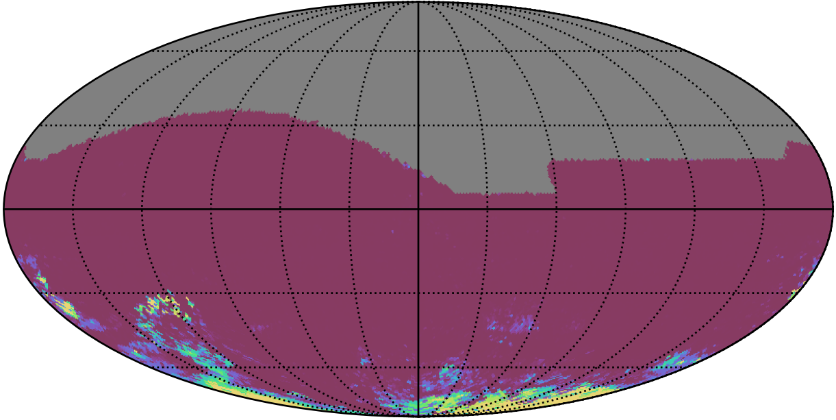
too_elab_r64_d2_giz_v3.4_10yrs All sky ri bands: 75th Percentile Intranight Timespan
