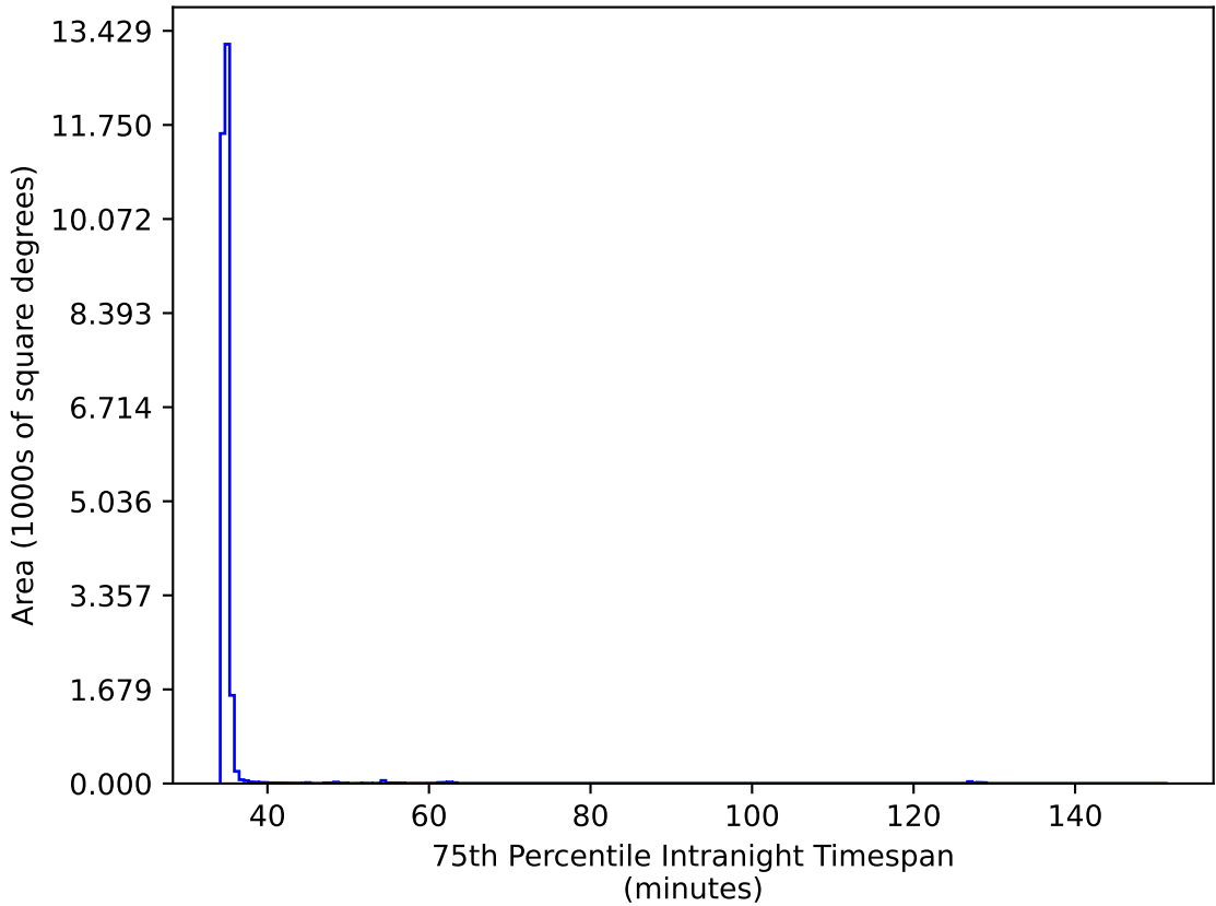
too_elab_r64_d2_giz_v3.4_10yrs All sky iz bands: 75th Percentile Intranight Timespan
