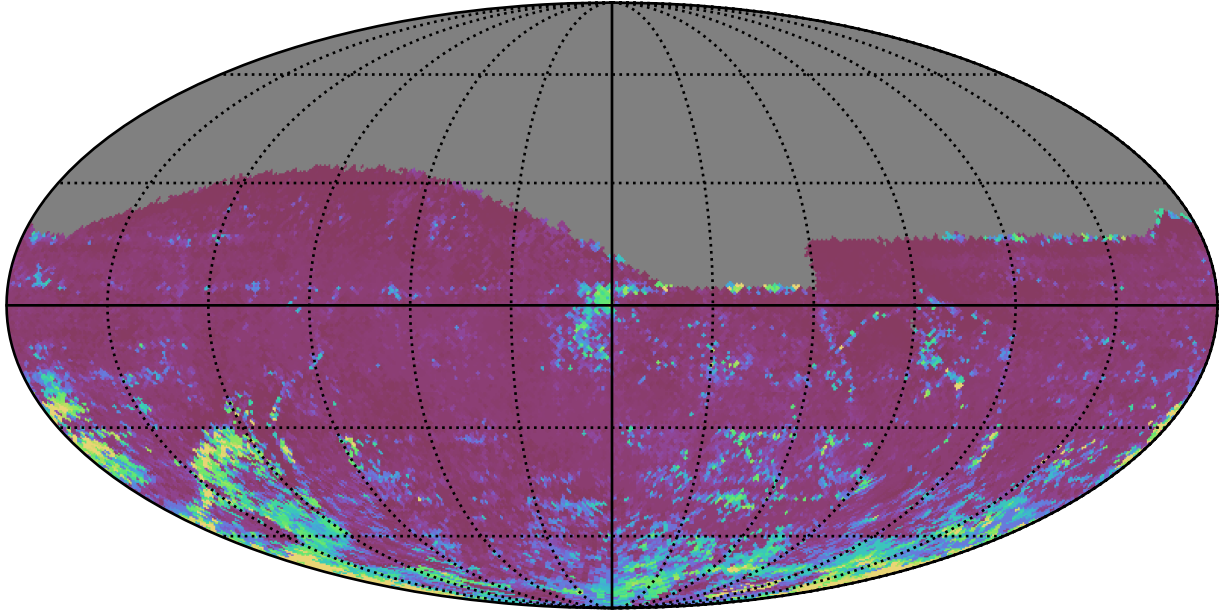
too_elab_r64_d2_giz_v3.4_10yrs All sky i band: 75th Percentile Intranight Timespan
