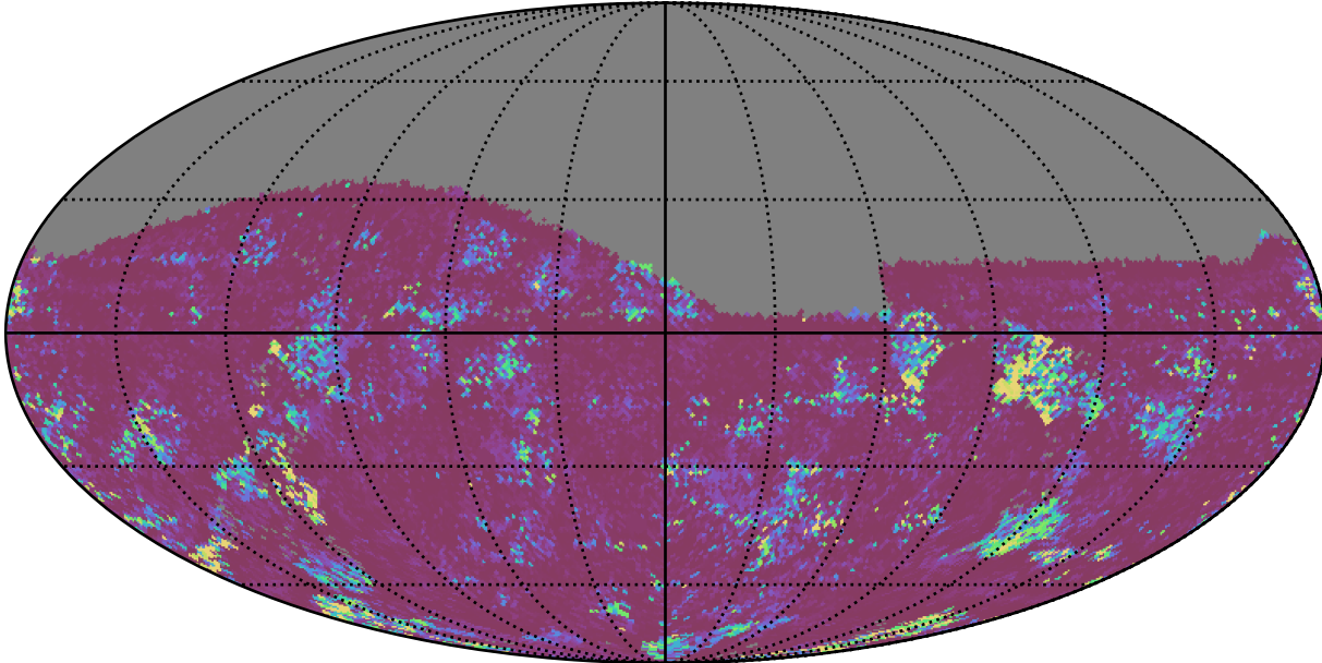
too_elab_r64_d2_giz_v3.4_10yrs All sky g band: 75th Percentile Intranight Timespan
