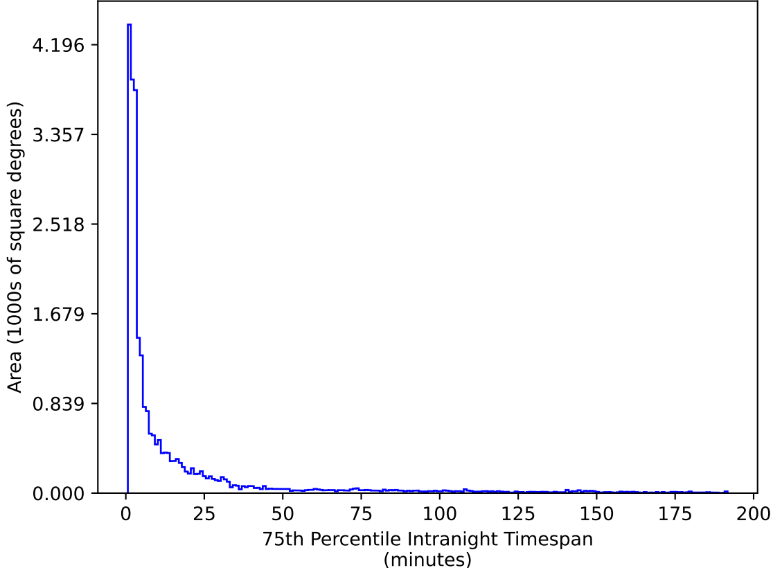
too_elab_r64_d2_giz_v3.4_10yrs All sky g band: 75th Percentile Intranight Timespan
