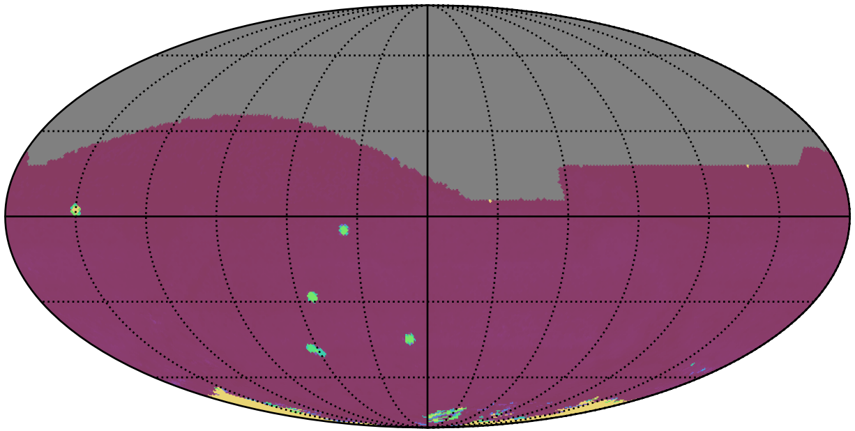
too_elab_r64_d2_giz_v3.4_10yrs All sky: 75th Percentile Intranight Timespan
