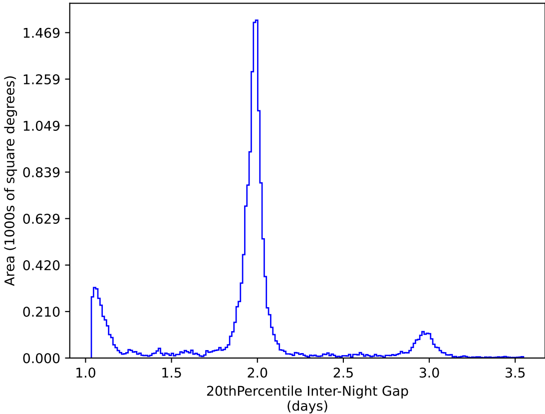
too_elab_r64_d2_giz_v3.4_10yrs WFD y band: 20thPercentile Inter-Night Gap
