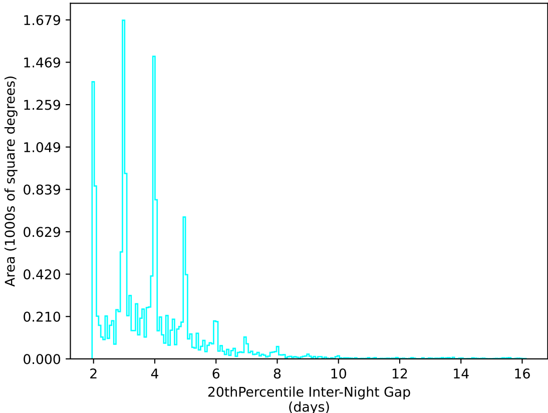
too_elab_r64_d2_giz_v3.4_10yrs WFD u band: 20thPercentile Inter-Night Gap
