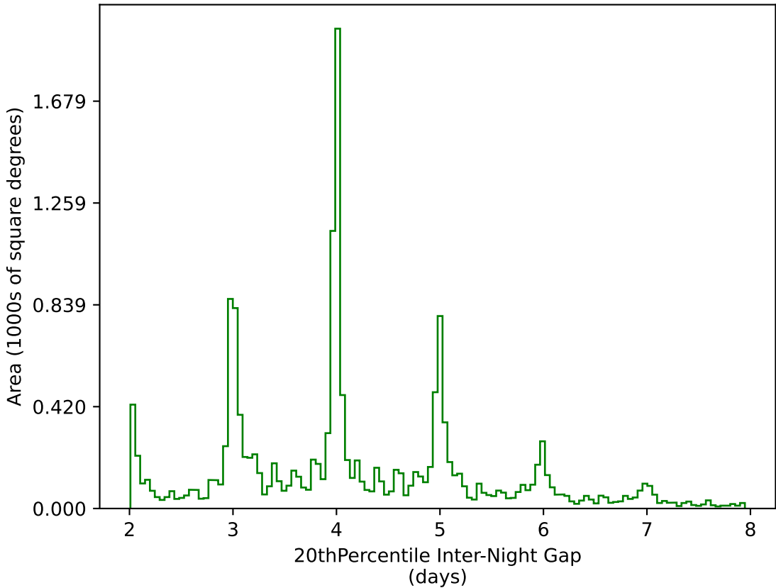
too_elab_r64_d2_giz_v3.4_10yrs WFD g band: 20thPercentile Inter-Night Gap
