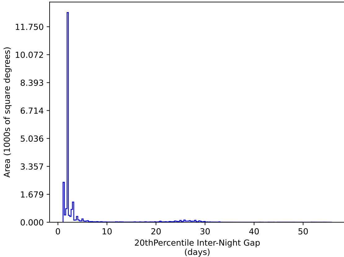
too_elab_r64_d2_giz_v3.4_10yrs All sky y band: 20thPercentile Inter-Night Gap
