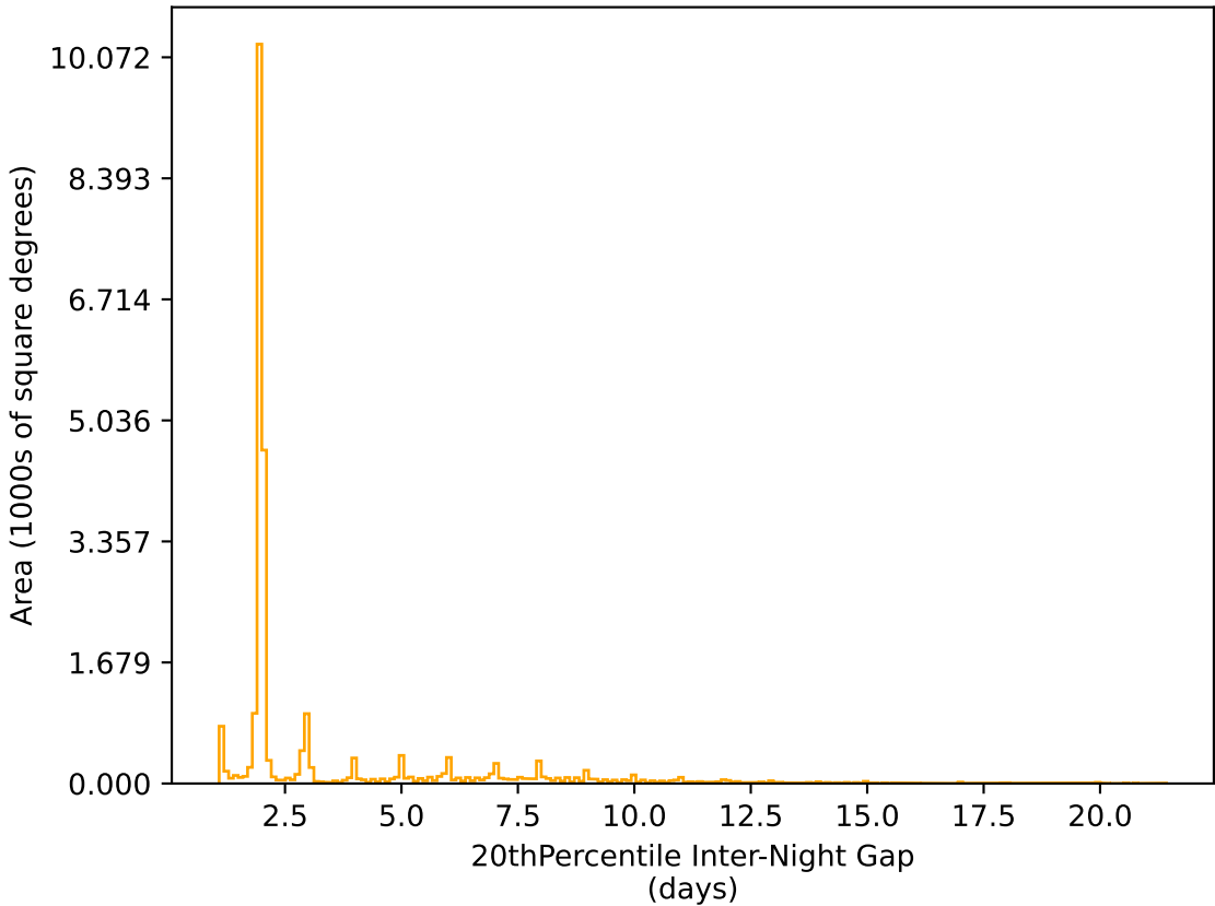
too_elab_r64_d2_giz_v3.4_10yrs All sky r band: 20thPercentile Inter-Night Gap
