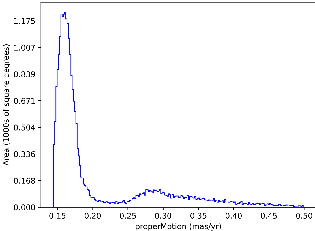
too_elab_r64_d2_giz_v3.4_10yrs : properMotion
